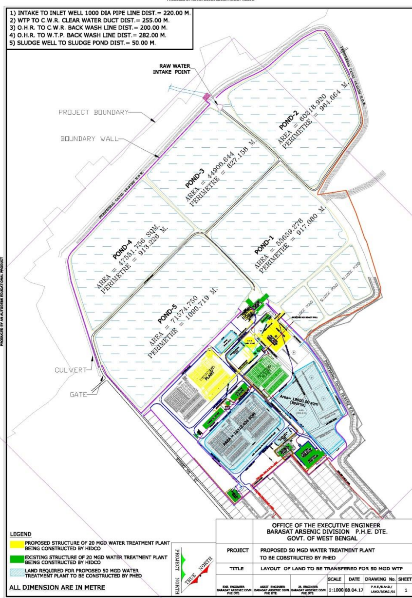
Figure 2: Layout Diagram of Proposed Water Treatment Plant
